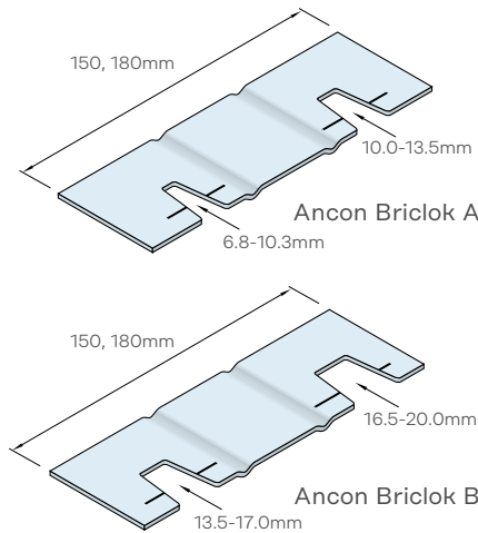
Ancon Staifix RT2 Wall Ties at 450mm vertical centres Ancon Briclok at 225mm vertical centres. Can be used in either leaf
