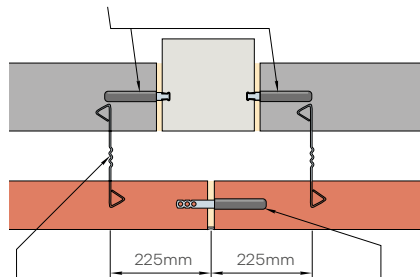
Ancon Staifix RT2 wall ties at 450mm vertical centres in alternate courses to PPS ties
