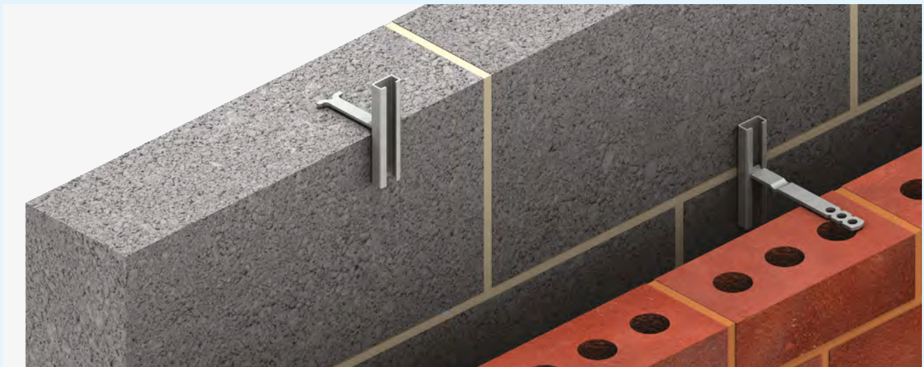
Ancon Fastrack Channels 100mm long with Ancon SD28 Tie
