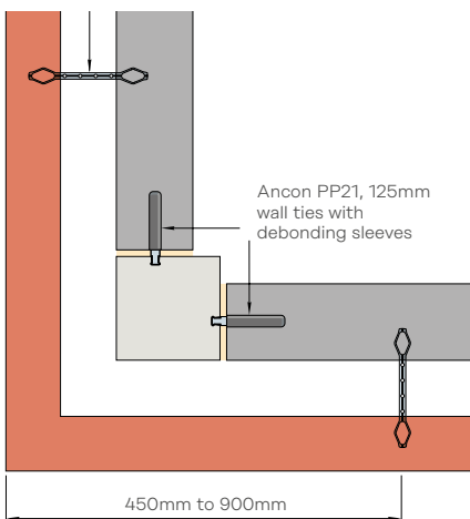
External Corner with Fully Bonded Brickwork
