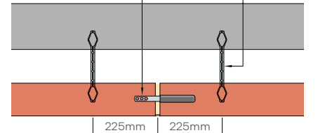
Cavity Wall with Vertical Movement Joint in Brickwork
