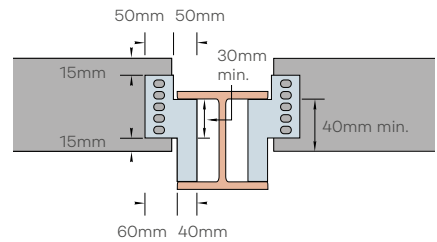
Non-Standard Ancon Internal Column Tie
