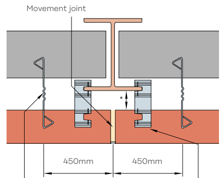
Ancon Staifix RT2 Wall Ties at 450mm vertical centres Ancon Briclok at 225mm vertical centres. Can be used in either leaf
