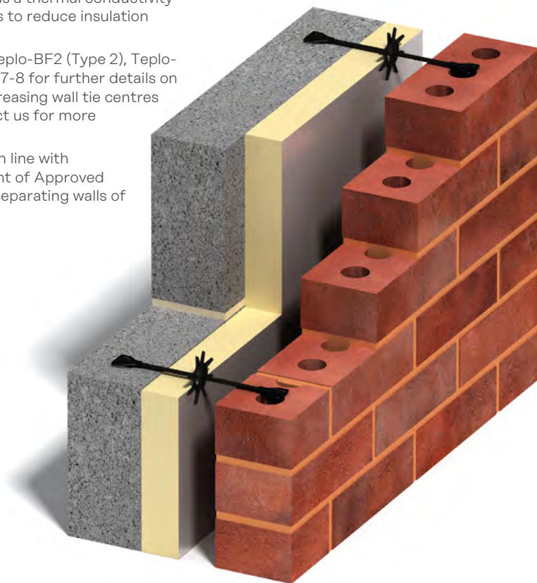
Ancon Teplo-BF is available in a range of diameters and lengths to suit cavities from 50mm to 450mm
